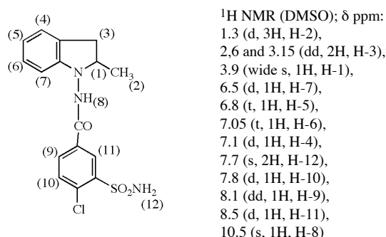
Figure 2. 1 H NMR data of Indapamide (1).
