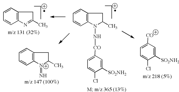
Figure 1. MS fragmentation of Indapamide (1).
